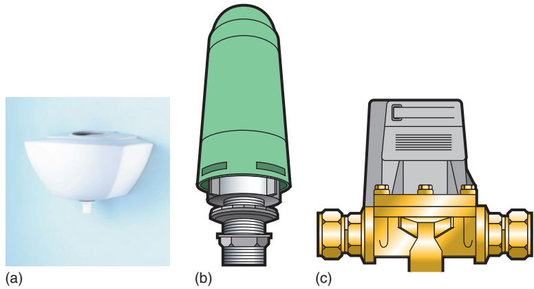
Figure 7.33 Automatic cistern and fittings (a) Cistern (Reproduced with permission of Ideal Standard Armitage Shanks), (b) Siphon, (c) Flushing valve
