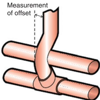
Figure 3.22 Pass-over offset
