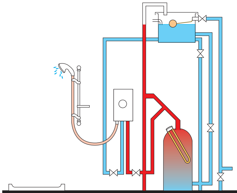
Figure 6.21 Installation details for a gravity fed shower using a shower pump (Reproduced with the kind permission of Mira Showers)
