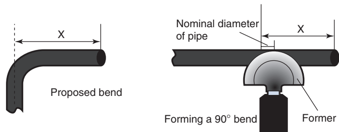
Figure 3.28 How to form a 90° bend
