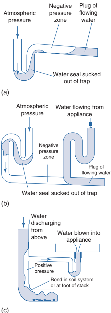
Figure 7.12 (a) Self-siphonage (b) Induced siphonage (c) Compression (Reproduced with permission of Hepworth Plumbing)
