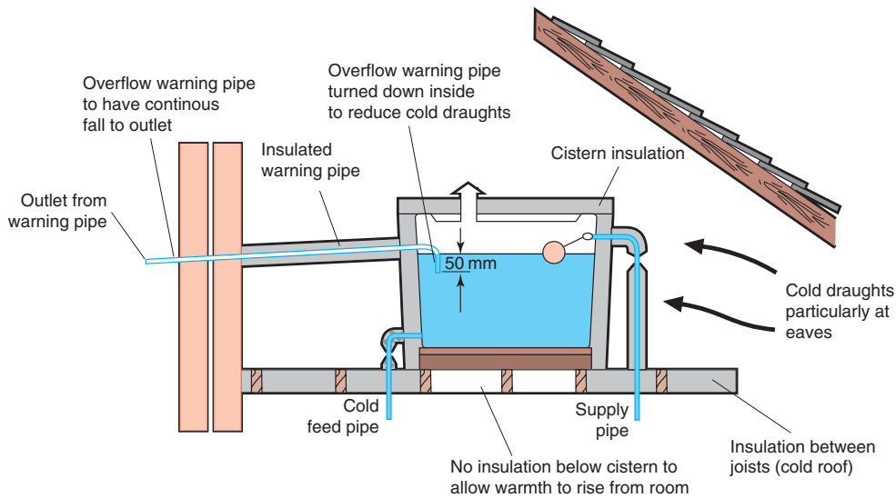
Figure 5.24 Details of insulated cold water storage cistern
