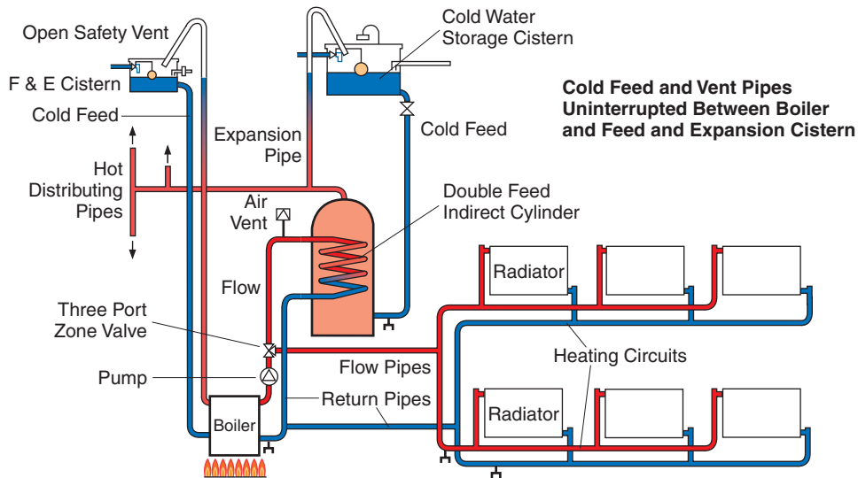
Figure 8.9 Fully pumped system
