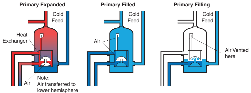
Figure 6.7 Single feed vessels
