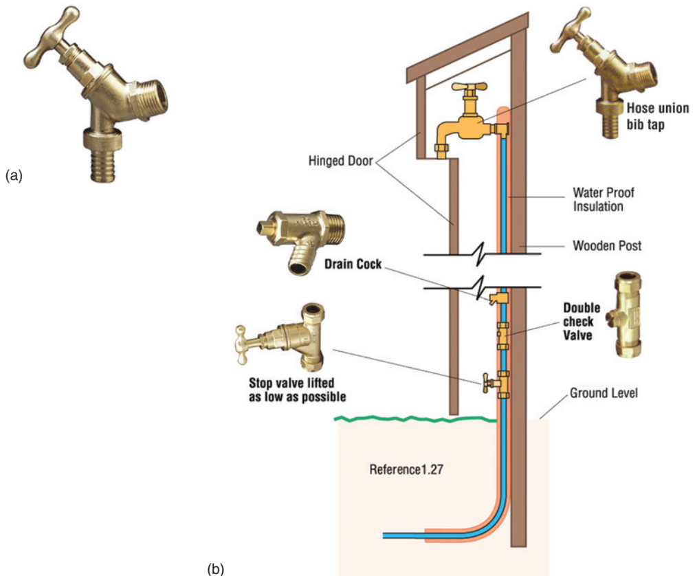
Figure 5.23 (a) Hose union bib tap (b) Requirements of external stand pipe
