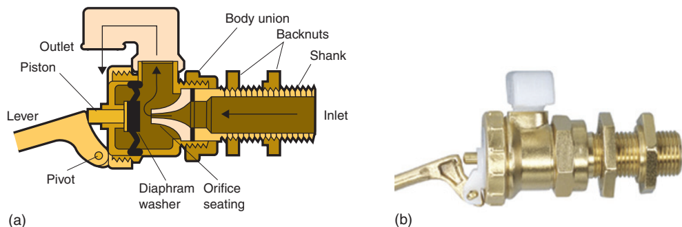
Figure 5.17 Diaphragm valve to BS 1212 Part 2 [(b) Reproduced with permission of Pegler Limited]
