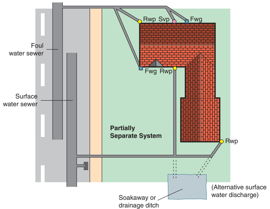
Figure 7.15 Partially separate system
