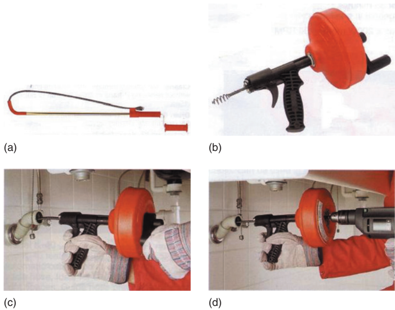
Figure 7.41 Range of mechanical equipment for clearing blockages (a) Closet auger, (b) Hand spinner, (c) Hand spinner in action clearing a wash basin waste pipe, (d) Power spinner with autofeed (Reproduced with permission for (b)–(d) from Ridgid Tool)
