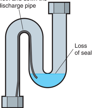
Figure 4.15 Loss of trap seal caused by capillary action
