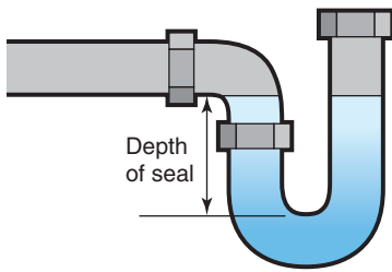
Figure 7.10 How to measure trap seal
