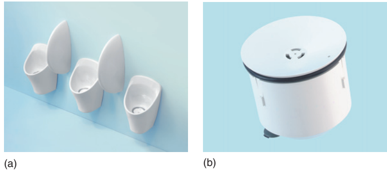
Figure 7.34 Waterless urinals (a) Typical urinal bowl installation, (b) Replaceable cartridges (Reproduced with permission of Ideal Standard Armitage Shanks)
