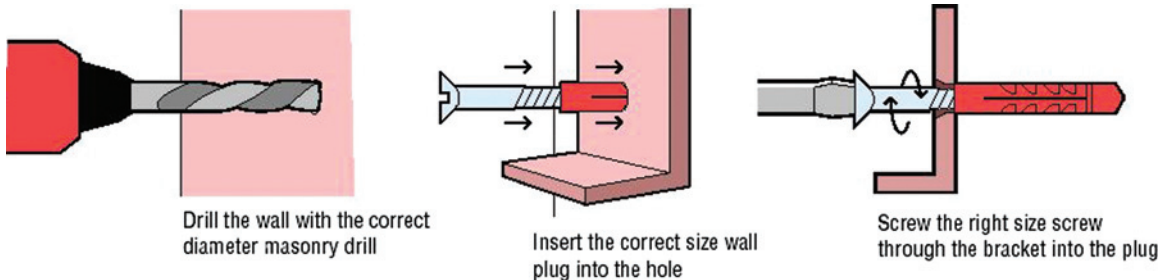
Figure 3.51 Fixing operation using plug and screw
