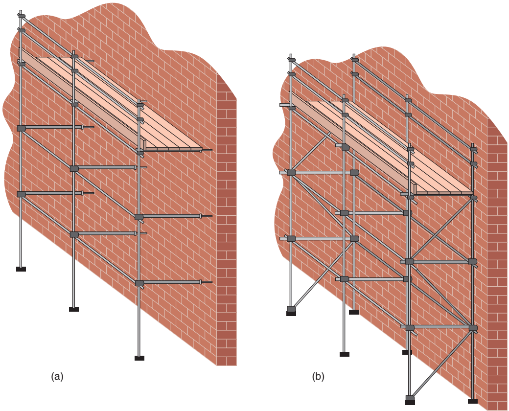
Figure 2.23 (a) and (b) Putlog and independent scaffolding
