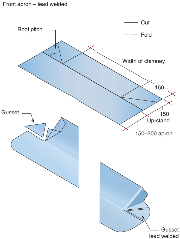
Figure 10.18 Welded part of apron (Reproduced with permission of Lead Sheet Association)
