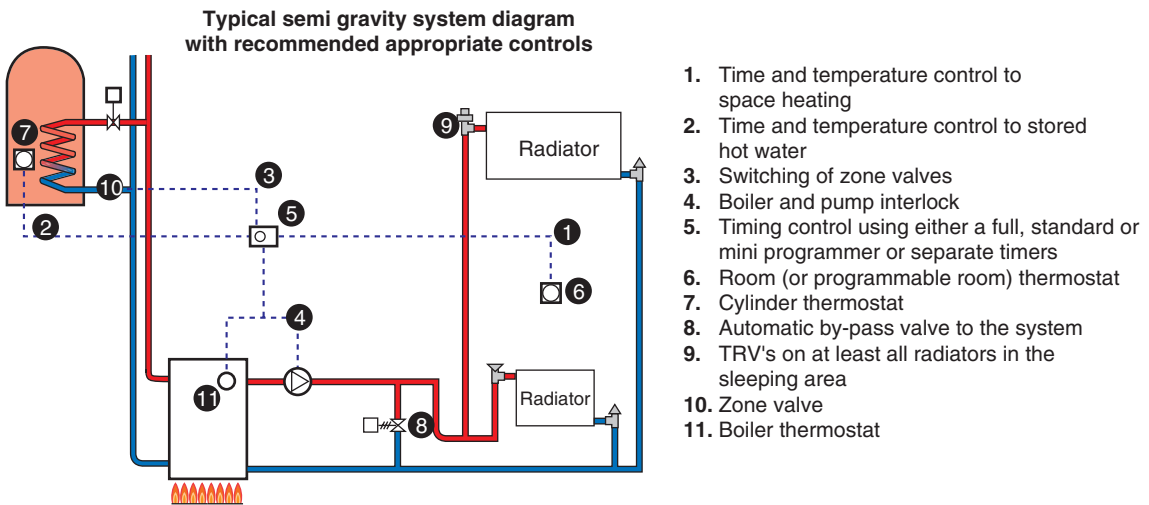
Figure 8.8 System meeting the requirements of Part L
