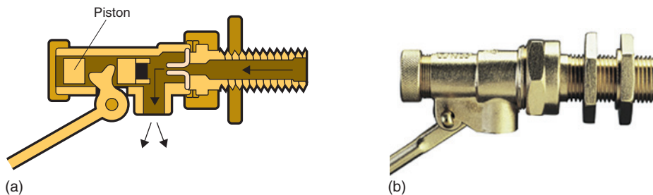
Figure 5.16 Portsmouth valve to BS 1212 Part 1 [(b) Reproduced with permission of Pegler Limited]
