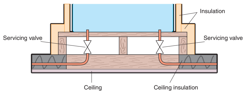
Figure 5.22 Requirements for suspended timber floors
