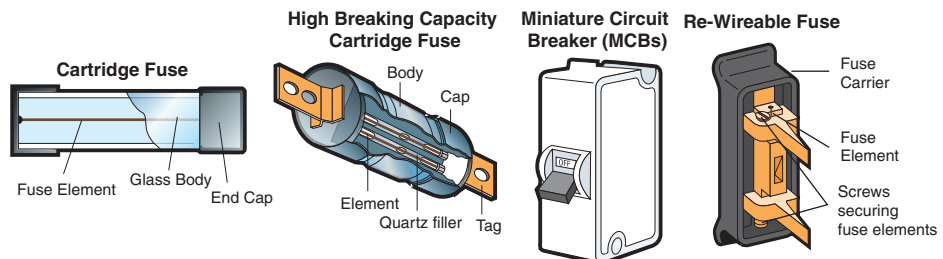
Figure 9.3 Types of fuses
