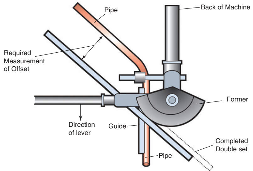
Figure 3.20 Pulling the offset
