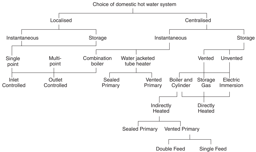
Figure 6.2 System selection flow chart
