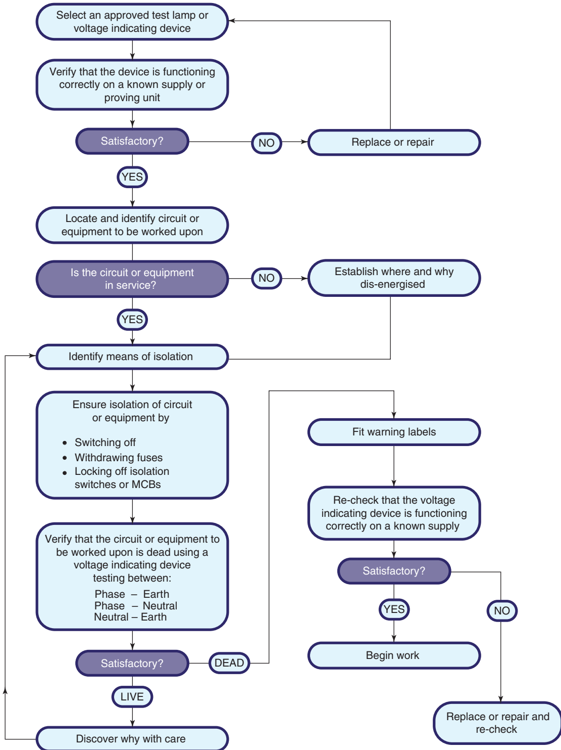
Figure 9.13 Isolation procedure
