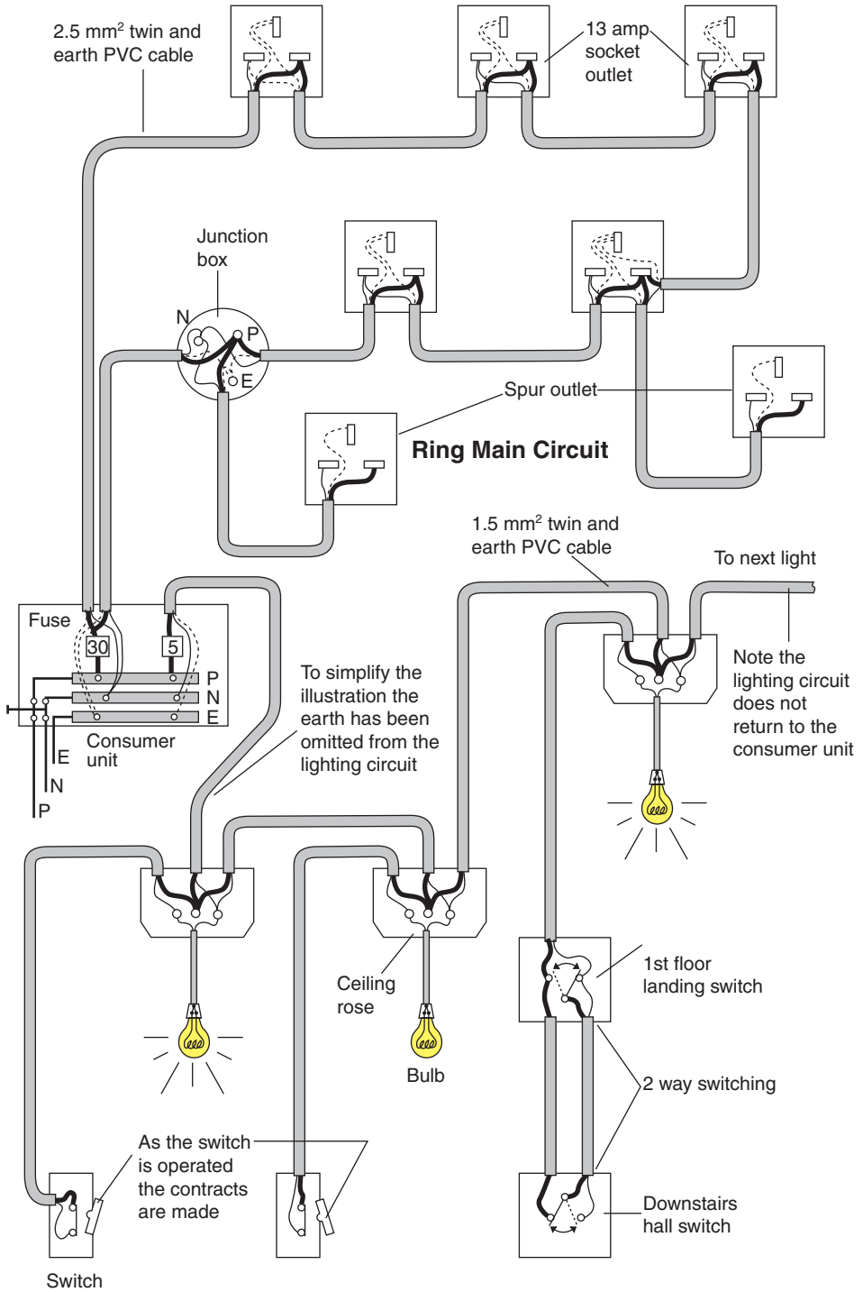
Figure 9.10 Lighting and ring main circuit
