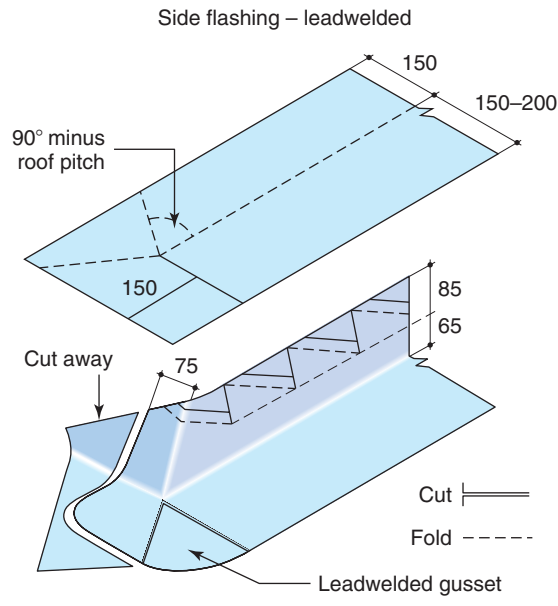
Figure 10.19 Side flashings lead welded (Reproduced with permission of Lead Sheet Association)
