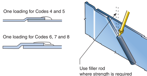
Figure 10.16 Inclined seam on vertical face (Reproduced with permission of Lead Sheet Association)
