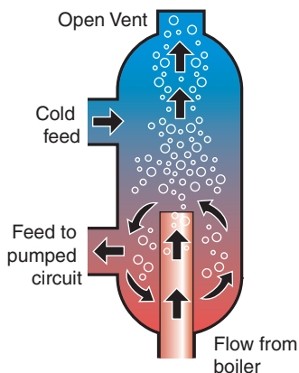
Figure 8.17 De-aerator
