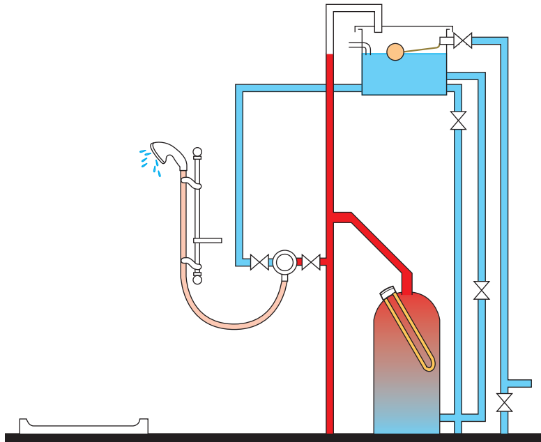
Figure 6.19 Installation details for a gravity fed shower with mixing valve (Reproduced with the kind permission of Mira Showers)
