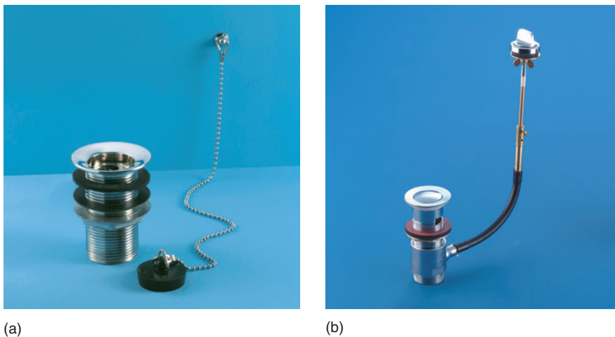
Figure 7.26 Waste fittings (a) Standard slotted-type, (b) Pop-up waste (Reproduced with permission of Ideal Standard Armitage Shanks)
