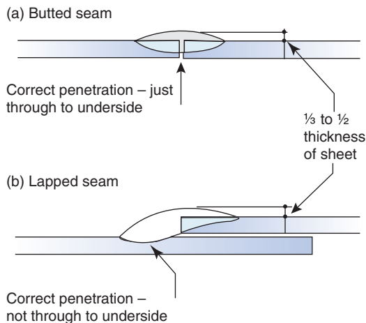
Figures 10.8 (a) and (b) Butted and lapped seam (Reproduced with permission of Lead Sheet Association)
