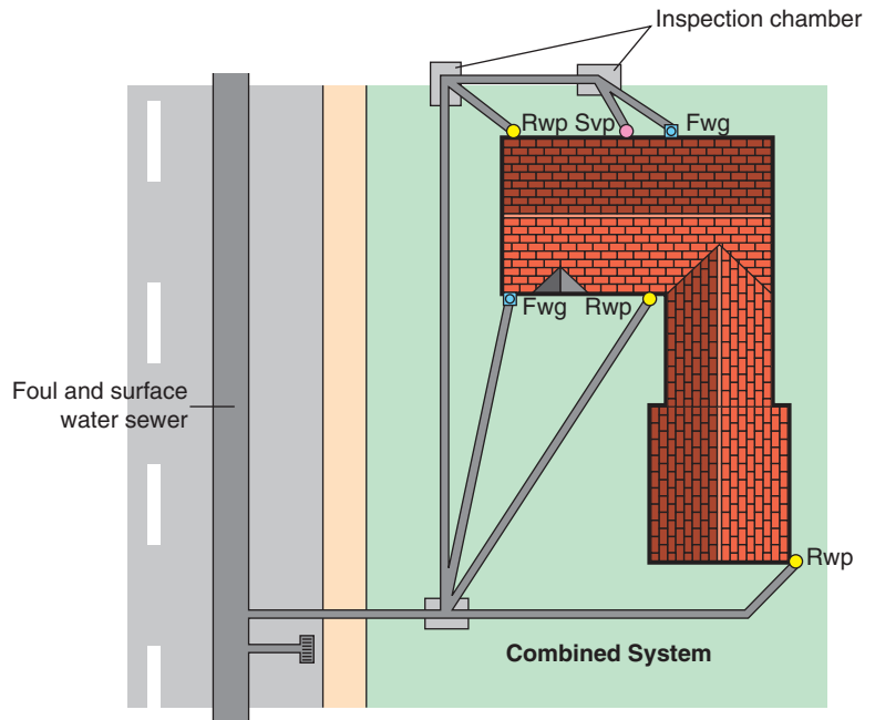
Figure 7.16 Combined System
