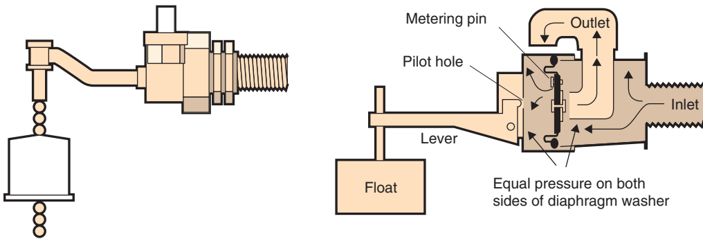
Figure 5.18 Diaphragm equilibrium float valves conforming to BS 1212 Part 4
