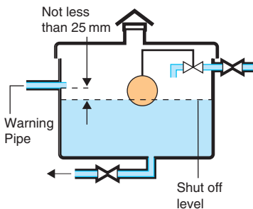
Figure 5.21 Warning pipe in a cistern with a capacity less than 1000l
