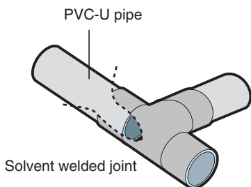
Figure 3.43 Section through solvent-welded joint
