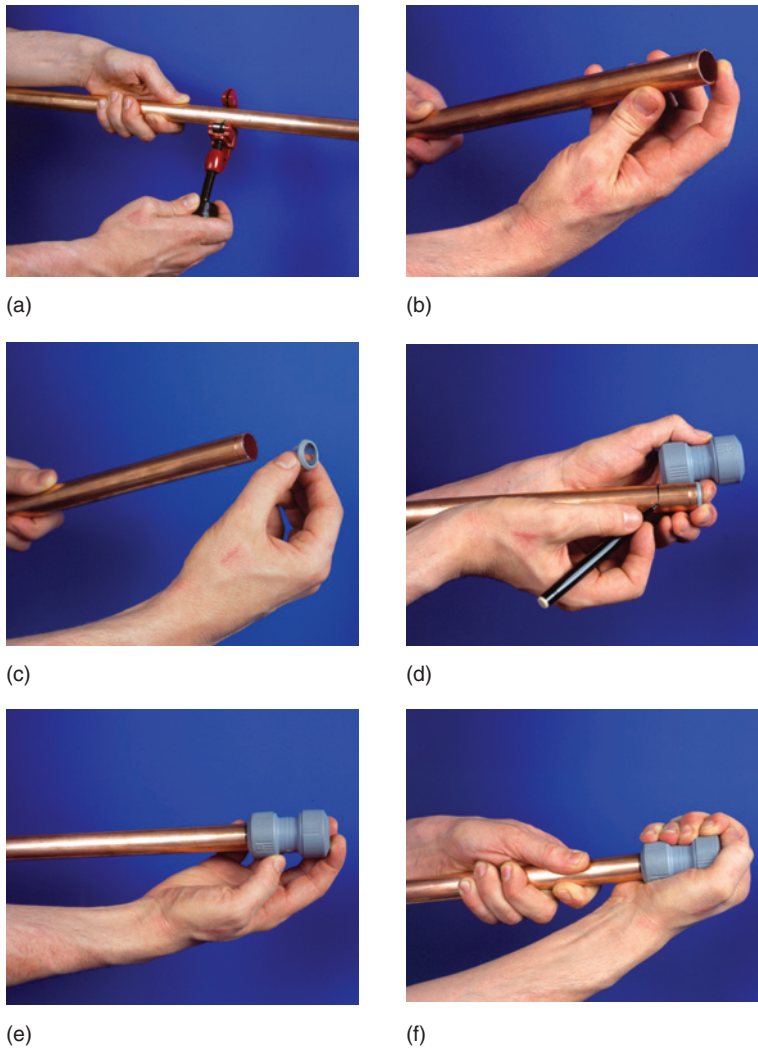
Figure 3.35 (a) Cut tube to length, (b) Clean and de-burr the pipe, (c) Insert ring to end of pipe, (d) Check pipe depth, (e) Fully push fitting into place, (f) Complete joint (Reproduced with permission of Hepworth Plumbing)
