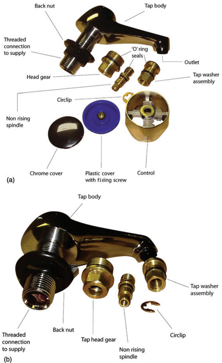
Figure 6.17 (a) Pillar tap components (b) Pillar tap seating and washer
