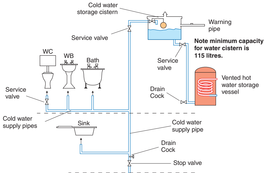
Figure 5.13 Direct system
