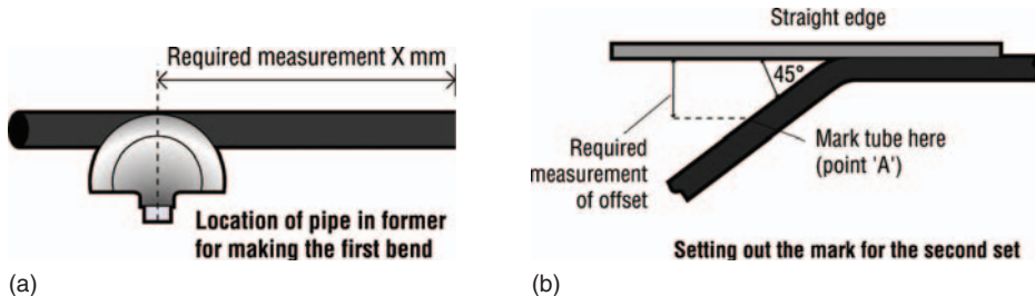
Figure 3.29 Low carbon steel offset
