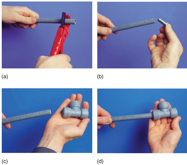
Figure 3.44 (a) Cut pipe to length and de-burr (b) Insert approved support liner (c) Position push fit fitting (d) Complete the joint (Reproduced with permission of Hepworth Plumbing)
