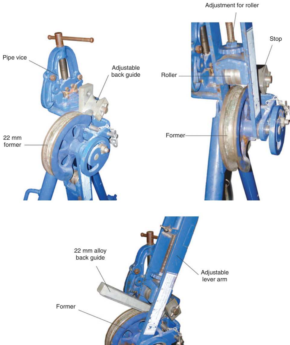
Figure 3.15 Components of a free-standing bending machine
