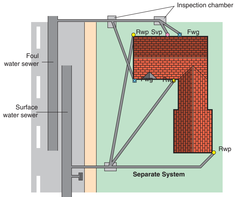
Figure 7.14 Separate System
