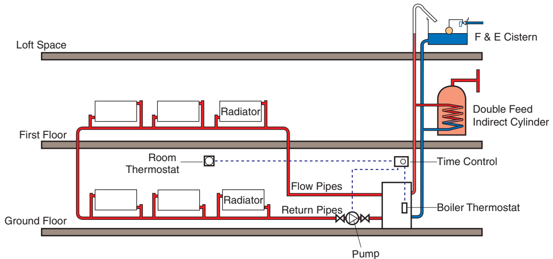
Figure 8.6 One-pipe system
