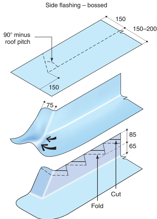
Figure 10.20 Side flashings bossed (Reproduced with permission of Lead Sheet Association)
