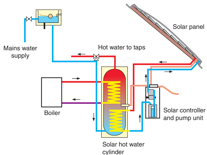
Figure 11.1 Solar-powered hot water system
