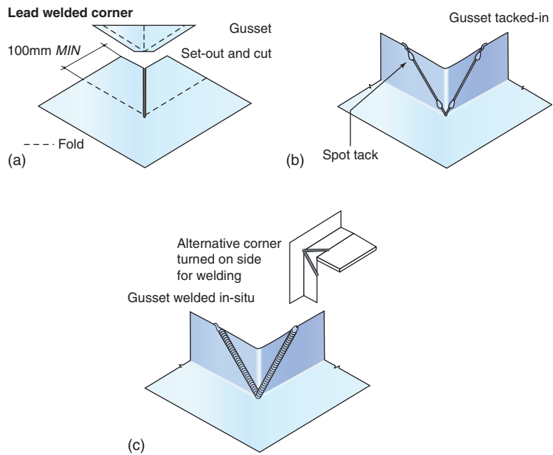
Figure 10.7 (a)–(c) Setting out for an external corner for welding (Reproduced with permission of Lead Sheet Association)
