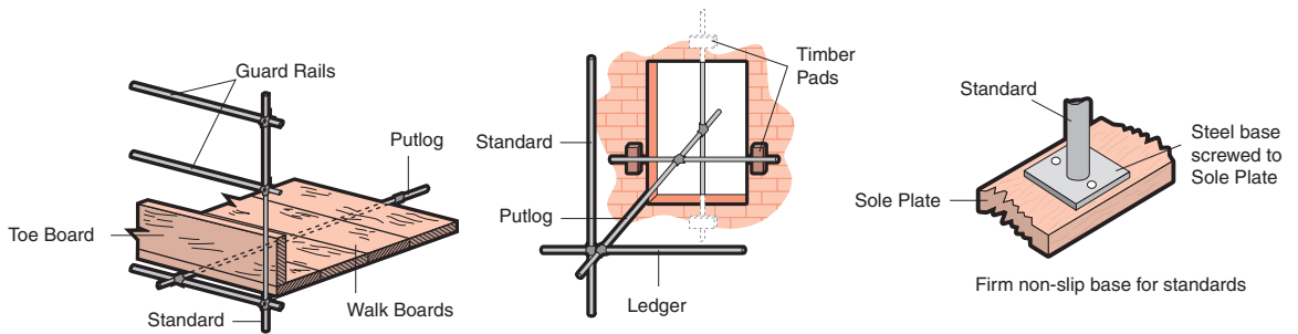
Method of tying scaffolds to a building through window or door openings
