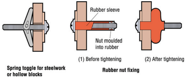
Figure 3.52 Spring toggle and rubber nut fixing
