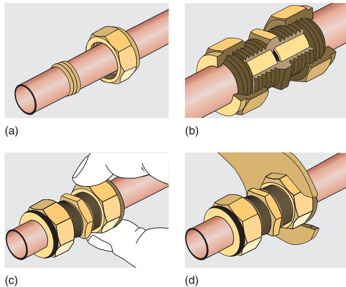
Figure 3.31 Non-manipulative jointing process (a) The pipe is cut to length and de-burred, and a nut and olive fitted, (b) Both pipe ends and olives are pushed home, (c) The nuts are hand tightened, (d) The joint is completed by tightening using a spanner or adjustable grips (Reproduced with permission of Pegler Limited)
