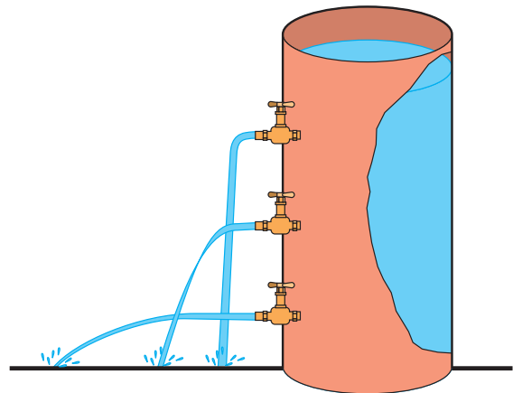
Figure 4.3 Water pressure
