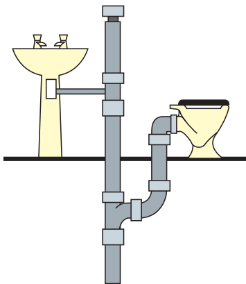
Figure 7.4 Use of air-admittance valves
