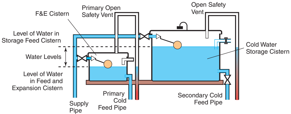
Figure 8.15 F&E cistern and CWSC arrangements
