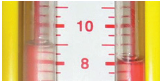
Figure 4.14 The meniscus
