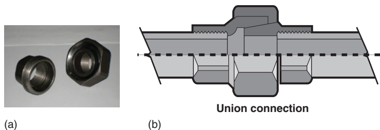
Figure 3.38 (a) Section through a male/female union (b) Section through union connection showing pipework
