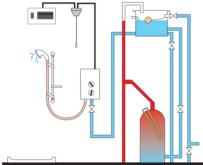
Figure 6.15 Electric instantaneous gravity fed shower (Reproduced with the kind permission of Mira Showers)
