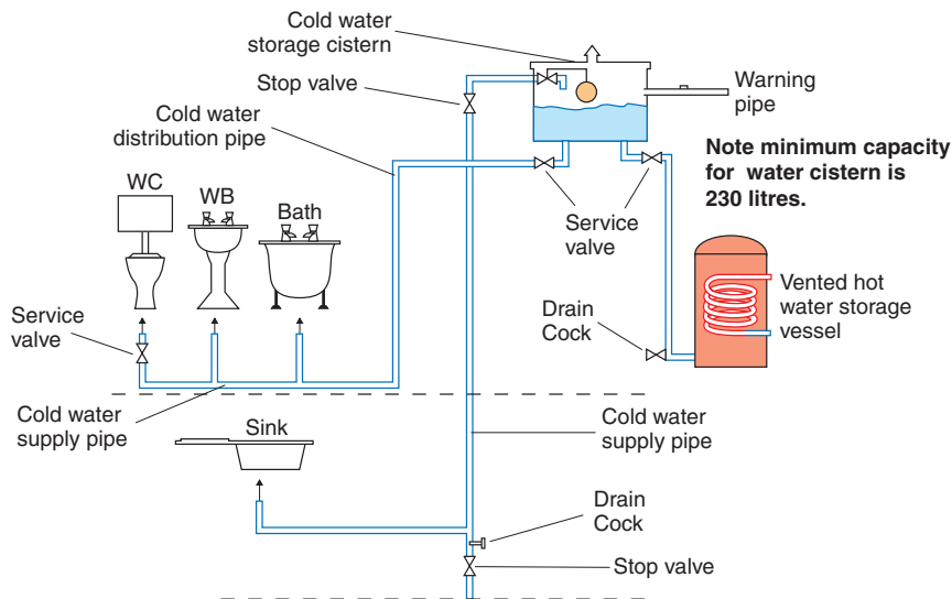
Figure 5.14 Indirect system
