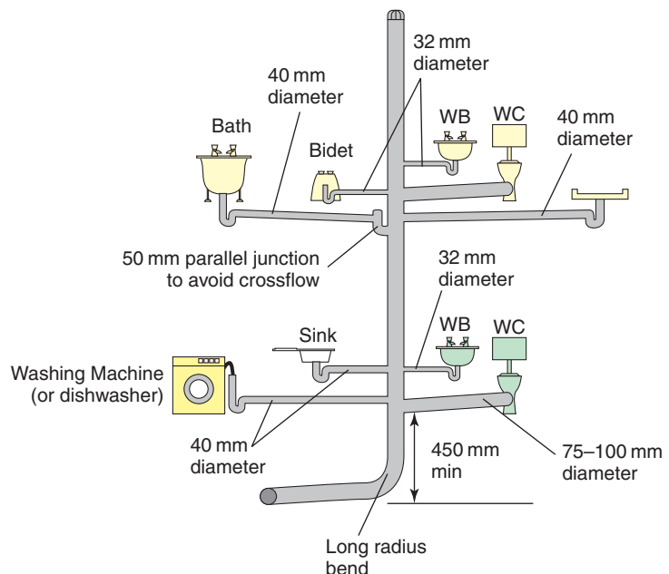
Figure 7.1 Primary ventilated stack
