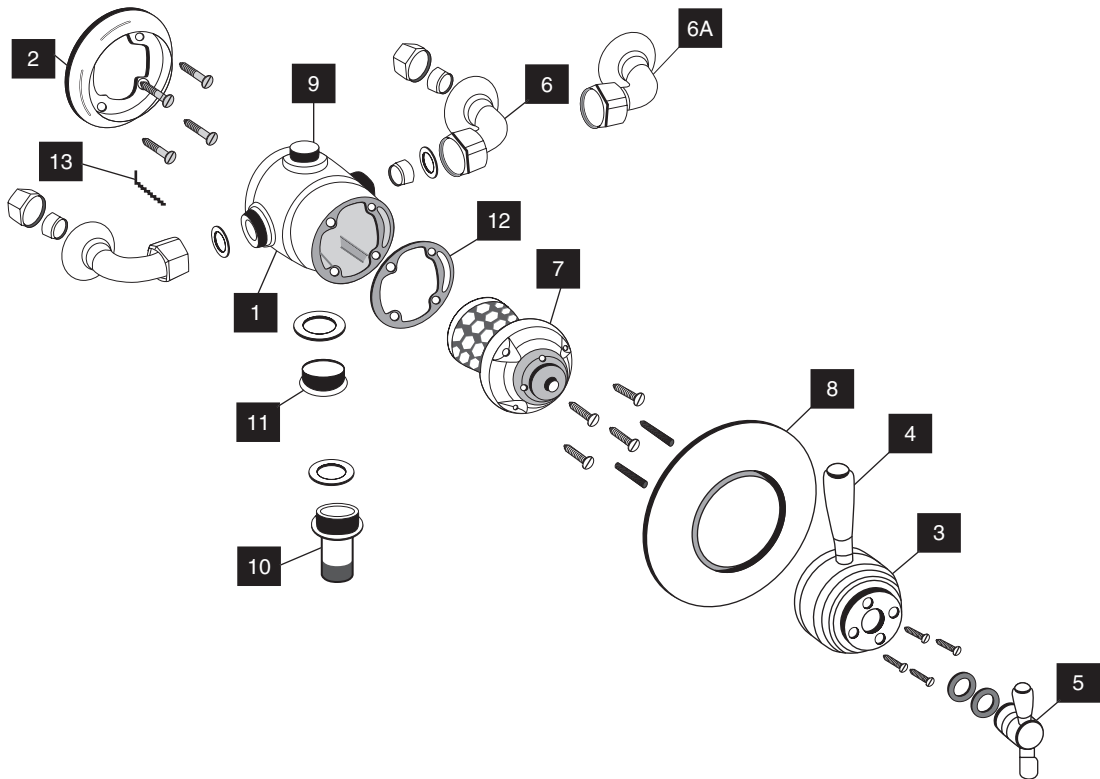
Figure 6.20 Exploded view of thermostatic shower mixer valve parts. List of components: 1. Shower body, 2. Wall mounting plate, 3. Temperature control lever, 4. Ceramic temperature control handle, 5. On/off control, 6. \frac{3}{4} " BSP elbow, 7. Thermostatic cartridge, 8. Wall plate, 9. \frac{3}{4} " outlet connector, 10. Hose connector, 11. Blanking plug, 12. Gasket with filter, 13. Allen key with grub screw
