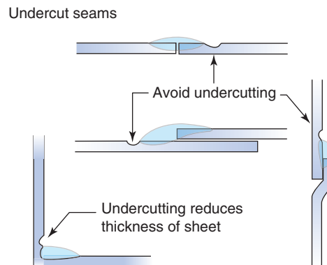
Figure 10.10 Undercutting (Reproduced with permission of Lead Sheet Association)
