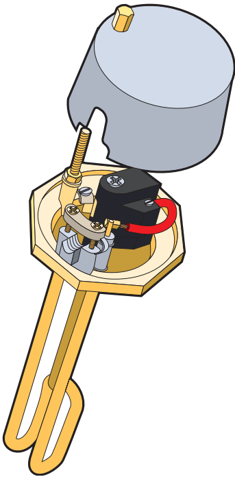
Figure 9.14 Immersion heater connections
