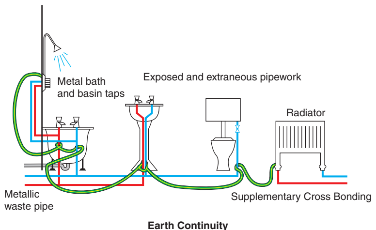
Figure 9.17 Earth continuity bonding
