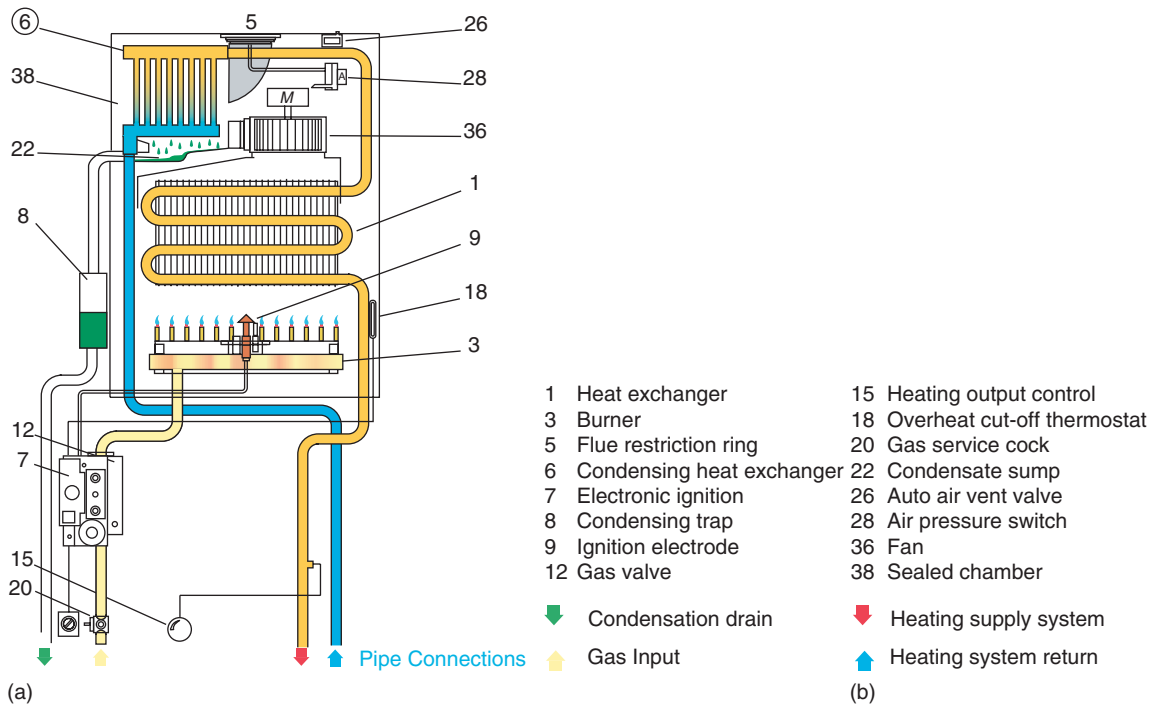
Figure 8.37 (a) and (b) Internal workings of the condensing boiler (Reproduced with permission of Ravenheat Manufacturing Limited)
