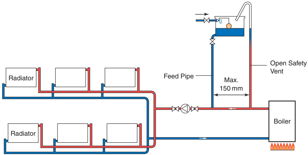
Figure 8.7 Two-pipe system
