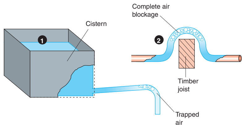
Figure 6.18 Common causes of air locks
