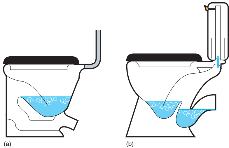
Figure 7.21 Siphonic pan (a) Single trap, (b) Double trap closed coupled
