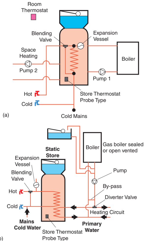
Figure 6.12 (a) Direct and (b) Indirect thermal stores
