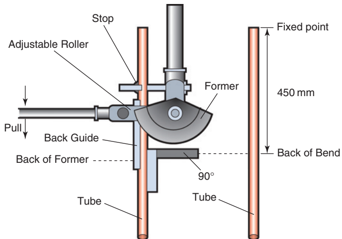
Figure 3.18 Tube Position in Former
