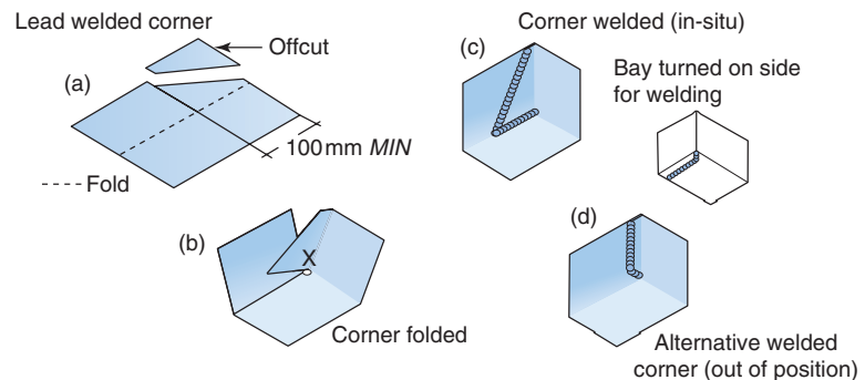
Figures 10.6 (a)–(d) Setting out for an internal corner for welding (Reproduced with permission of Lead Sheet Association)
