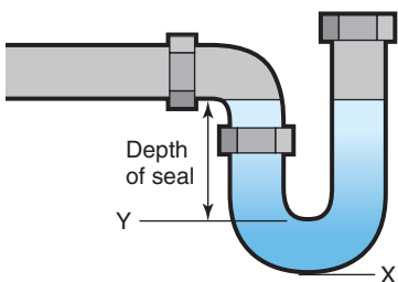
Figure 7.38 Measuring depth of seal
